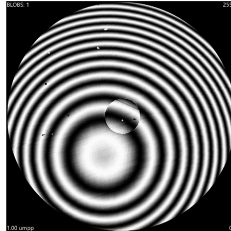
Interferometer view
